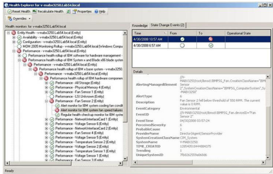
Figure 47. Example of a knowledge page that describes an error event
