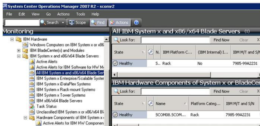
Figure 30. Dashboard view
