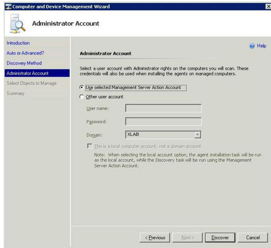
Figure 39. Administrator Account
