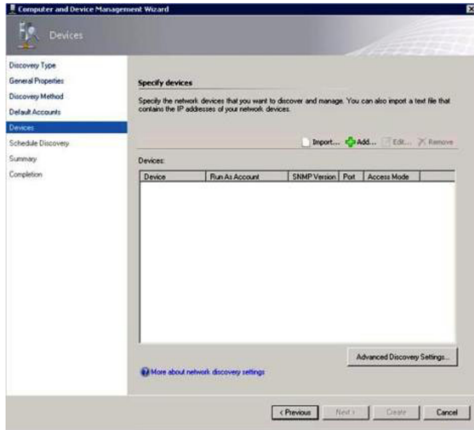
Figure 12. Devices page
