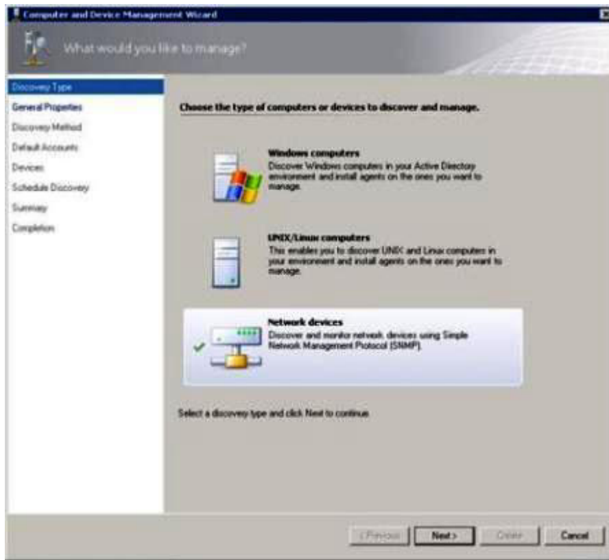
Figure 9. Discovery types
